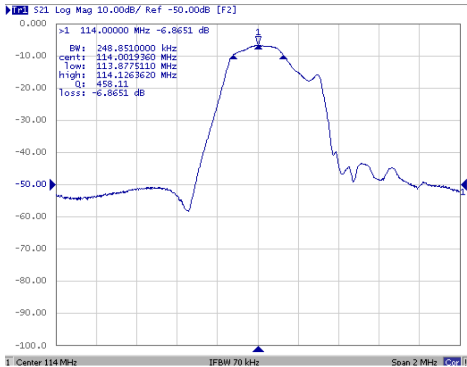
Fig1. Horizontal: 0.2MHz/Div Vertical: 10dB/Div
