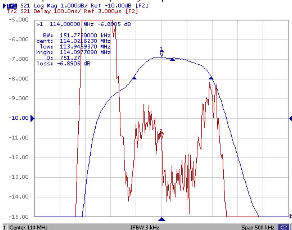
Fig2. Horizontal: 0.05MHz/Div Vertical: 1dB/Div Vertical: 100ns/Div
